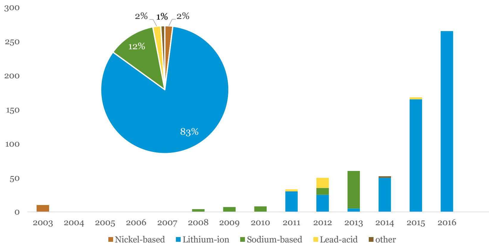
Large-scale battery storage capacity by type (megawatt hours and percent total)
